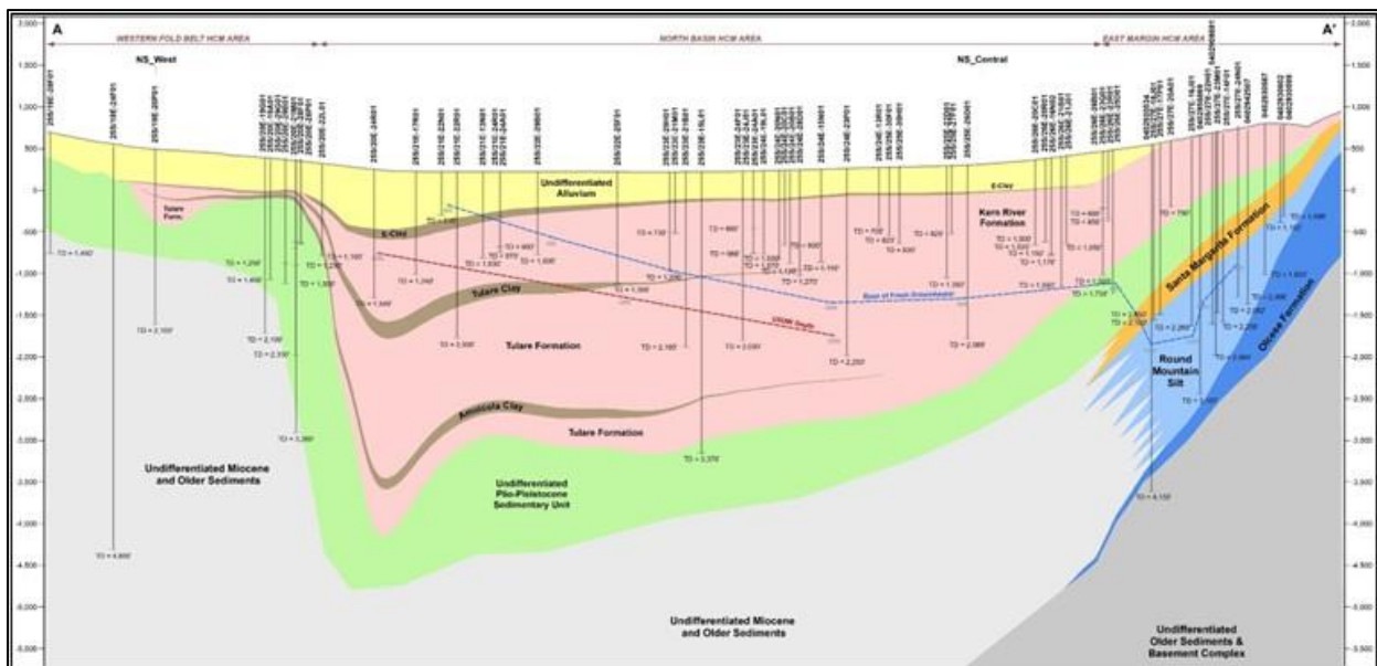
Figure ES-4. Subbasin Cross Section
