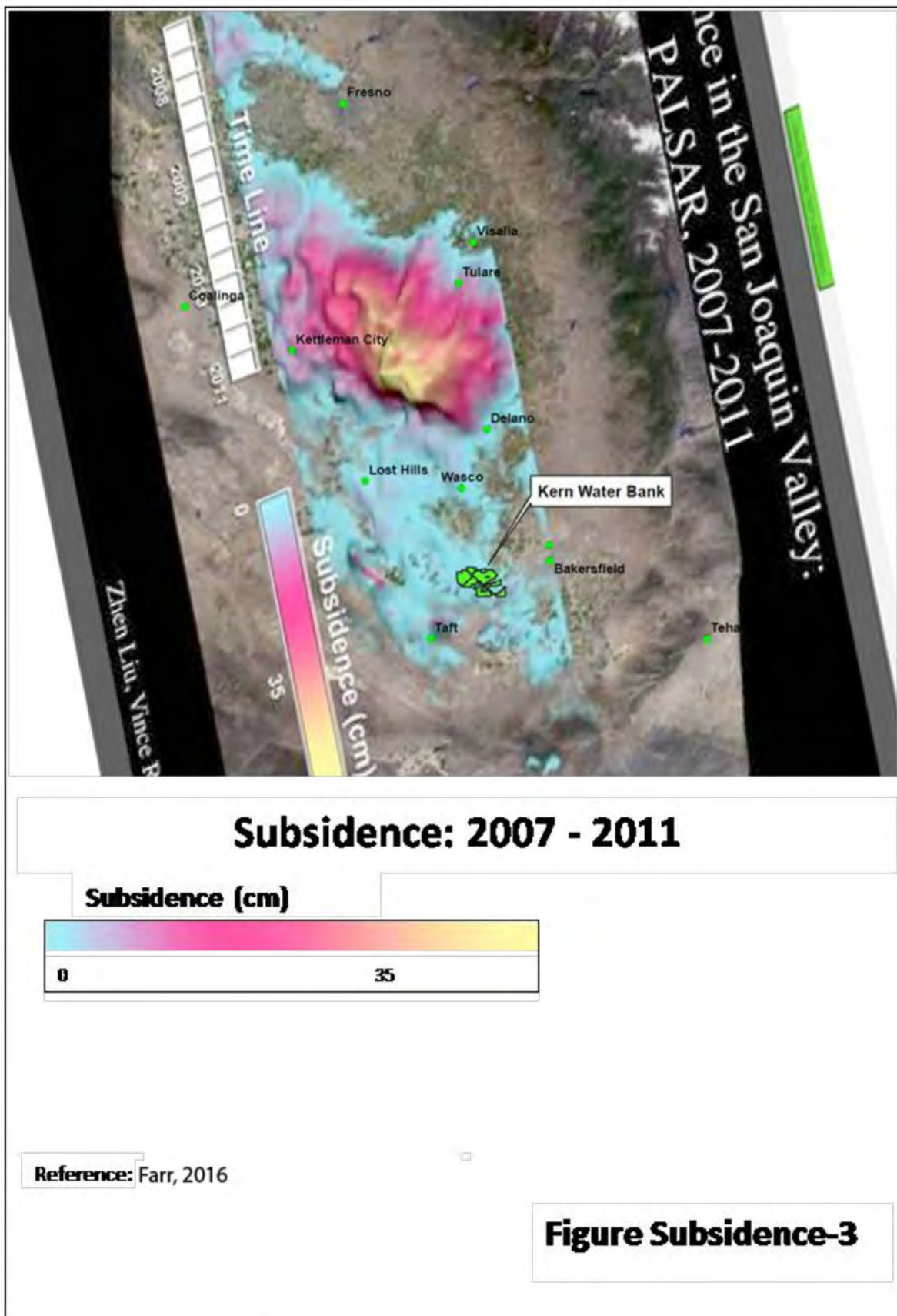
Figure 4-9. Subsidence: 2007-2011
