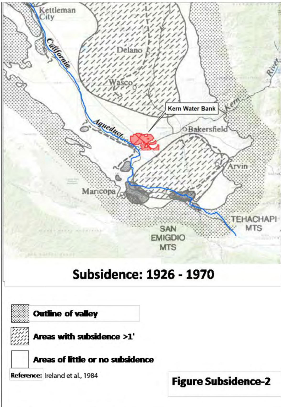
Figure 4-8. Subsidence: 1926-1970
