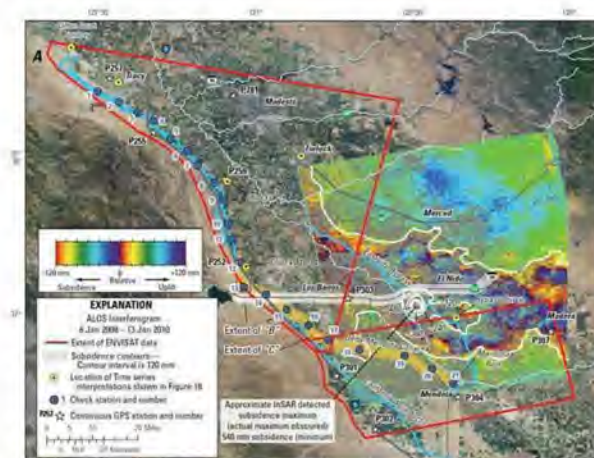
(ALOS interferogram with subsidence contours showing vertical changes in land surface in the central San Joaquin Valley area, California, during January 8, 2008–January 13, 2010)
