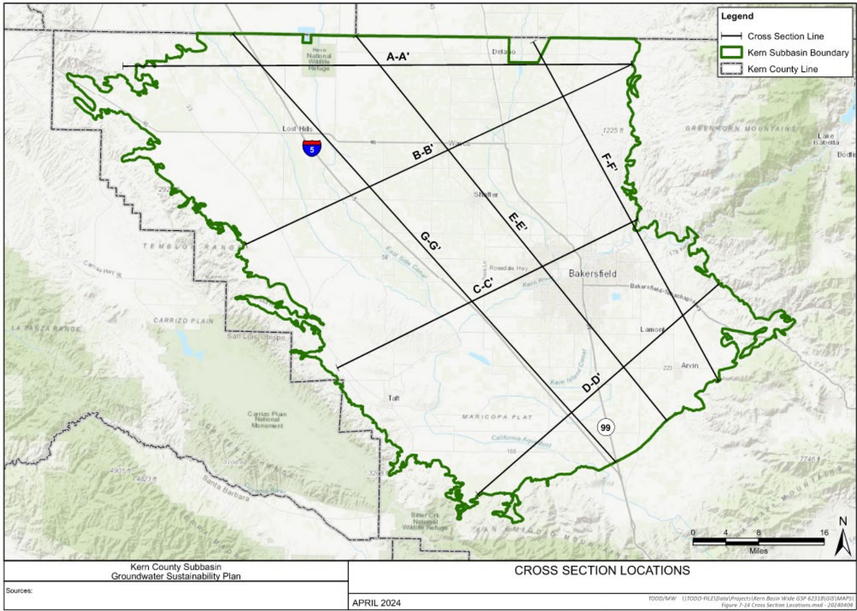
Figure BF-2. Cross Section Locations.
