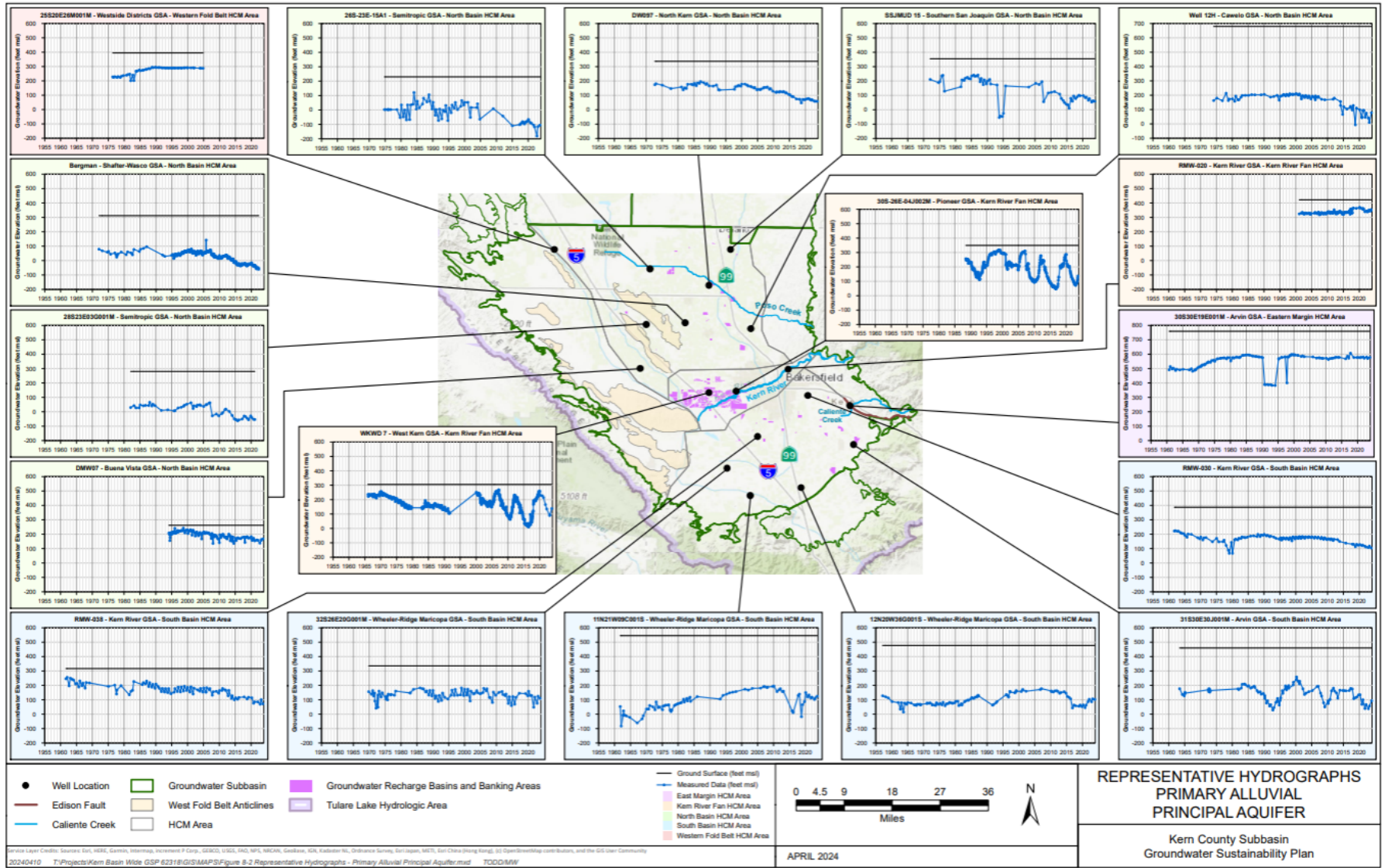
Figure BF-9. Representative Hydrographs Primary Alluvial Principal Aquifer.
