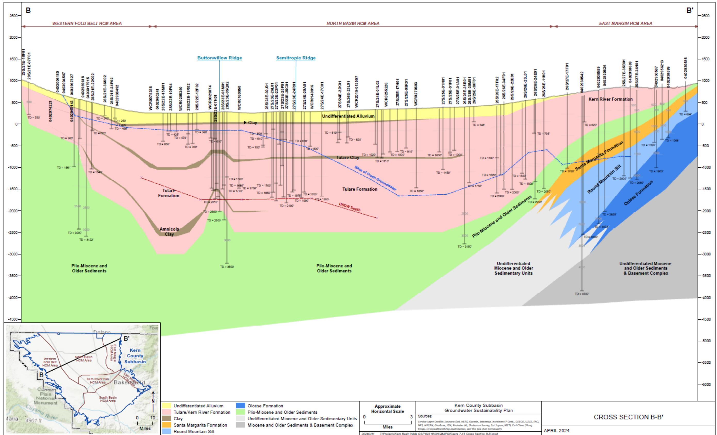
Figure 7-16. Cross Section B-B'
