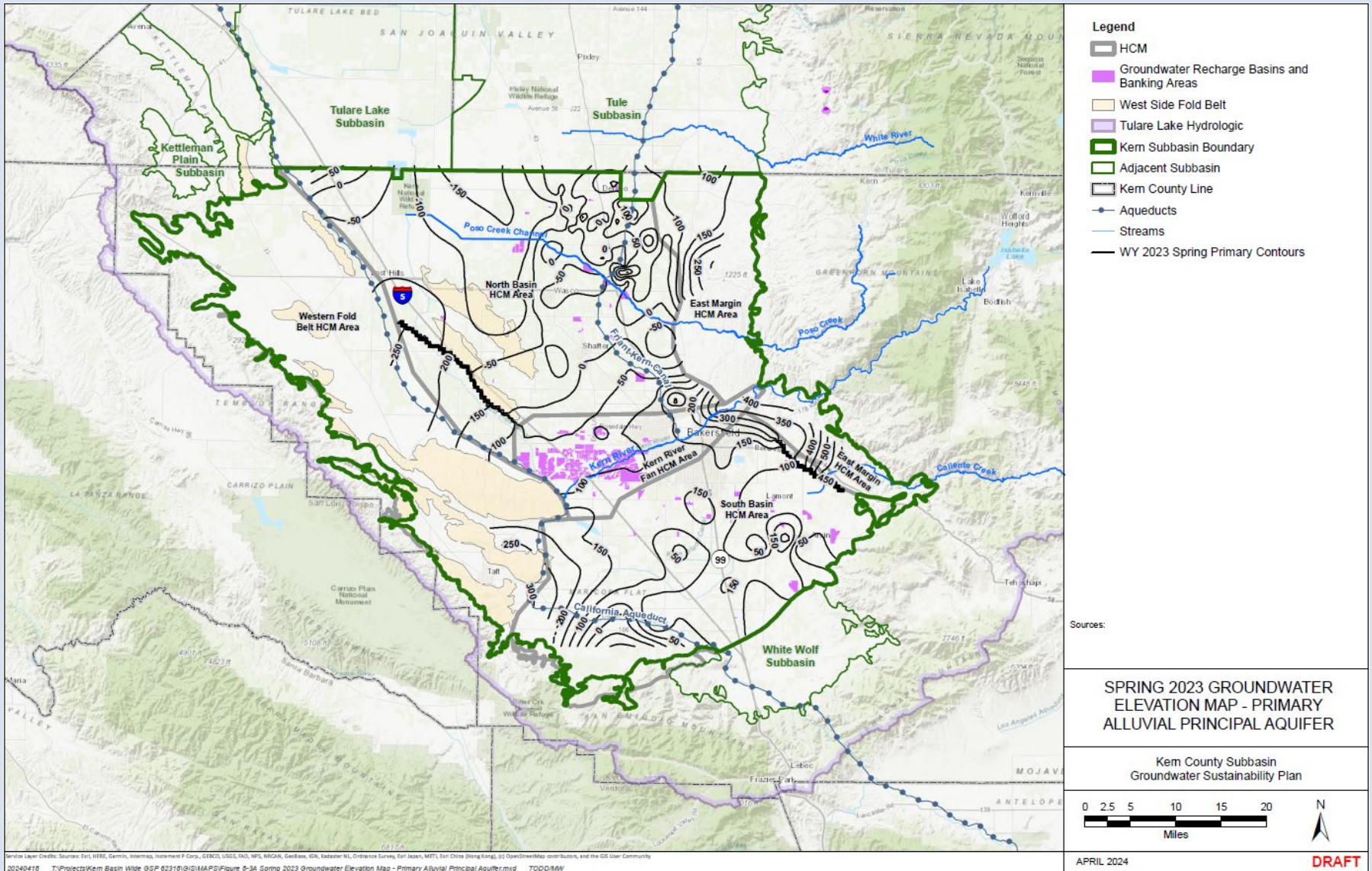
Figure BF-7. Spring 2023 Groundwater Elevation Map – Primary Alluvial Principal Aquifer.
