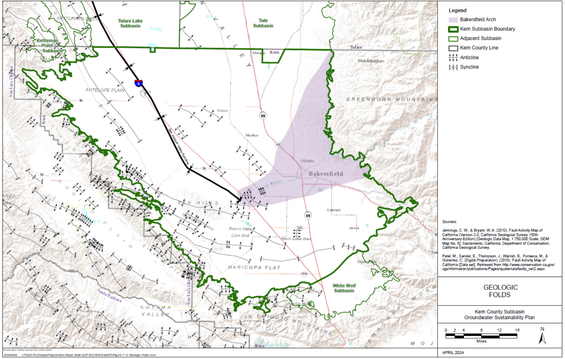
Figure BF-5. Geologic Folds.
