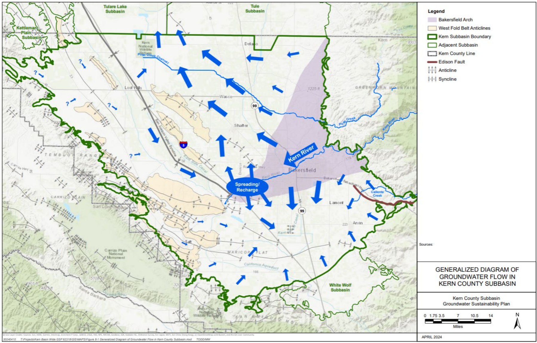
Figure BF-6. Generalized Diagram of Groundwater Flow in Kern County Subbasin.
