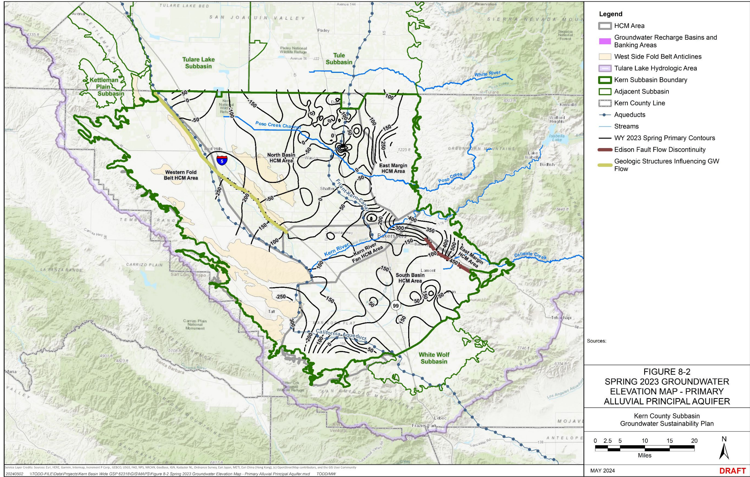
Figure 8-2. Spring 2023 Groundwater Elevation Map – Primary Alluvial Principal Aquifer
