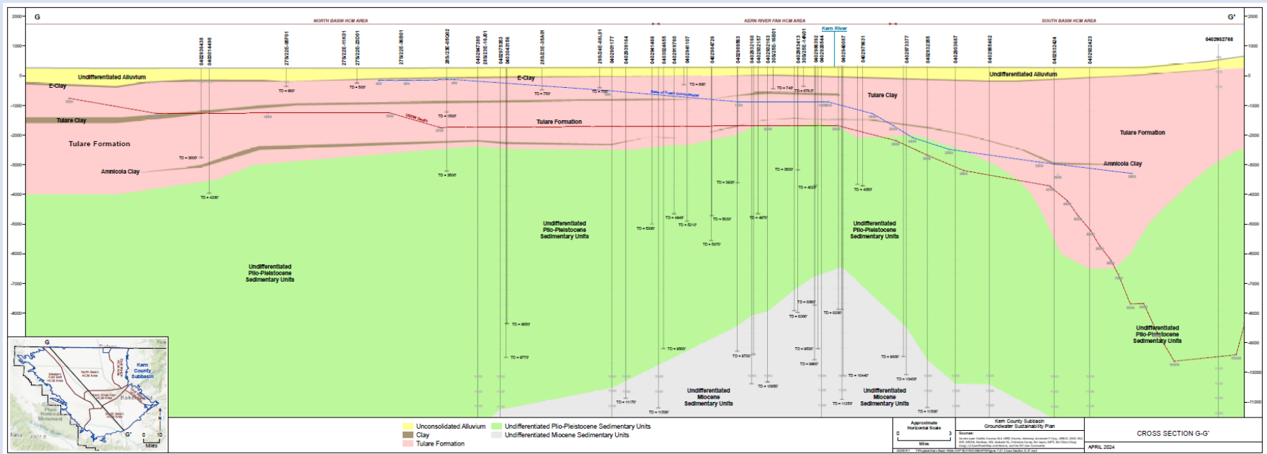
Figure BF-3. Cross Section G-G'.
