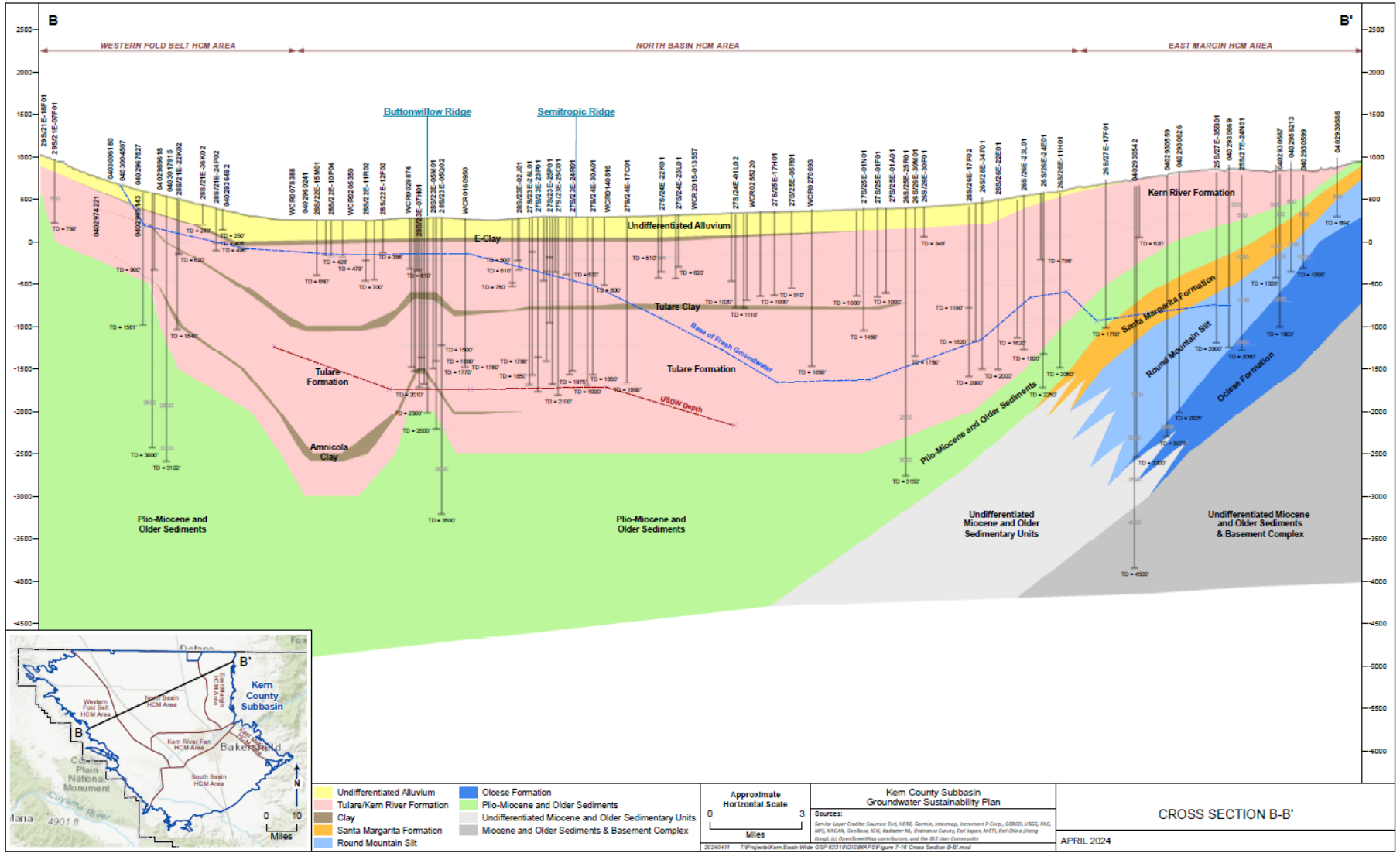
Figure BF-4. Cross Section B-B'.
